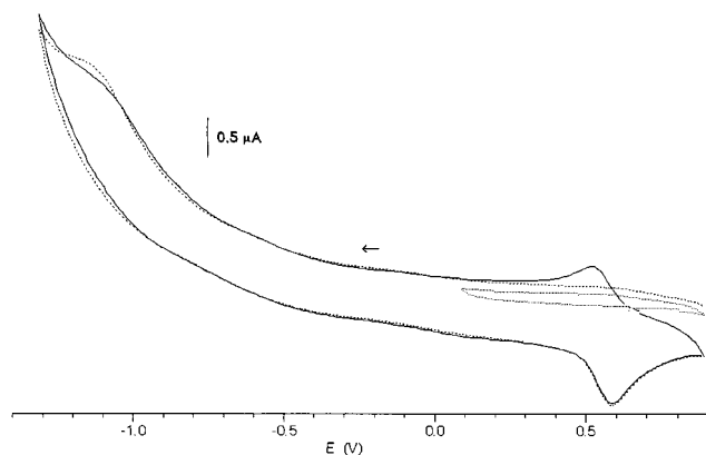
Figure 6. Comparison of results from cathodic cyclic voltammetric scans for [\text{Ru}(4,4'\text{-C}=\text{CHC}_6\text{H}_4\text{C}\equiv\text{CPh})\text{Cl}(\text{dppm})_2]\text{PF}_6 ( 14 ) using switching potentials of -1.4 (two successive scans) and 0 V.
